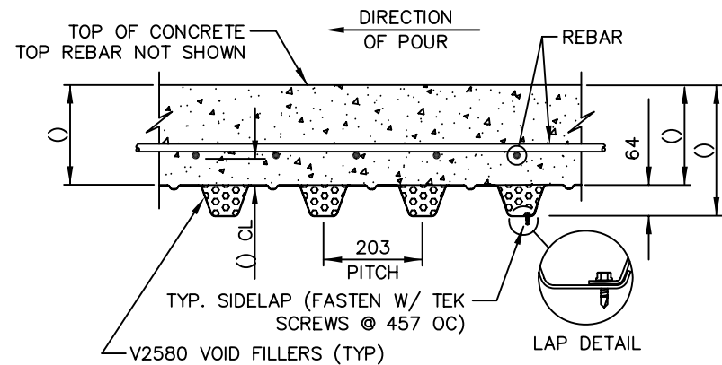
64 x 203 SLAB SECTION
