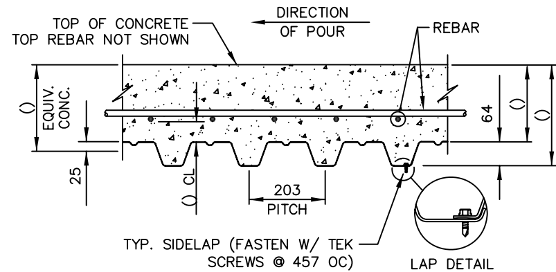
64 x 203 SLAB SECTION
