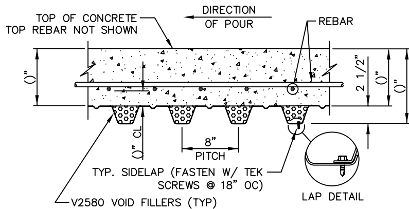
2 1/2" x 8" SLAB SECTION
