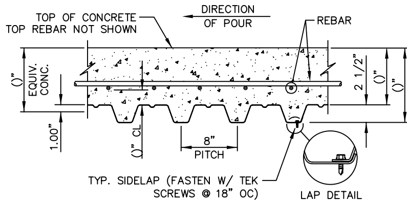
2 1/2" x 8" SLAB SECTION
