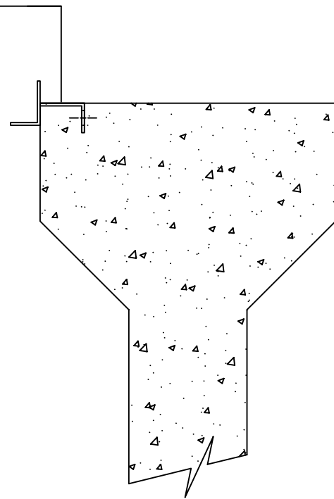
EXTERIOR BEAMS
