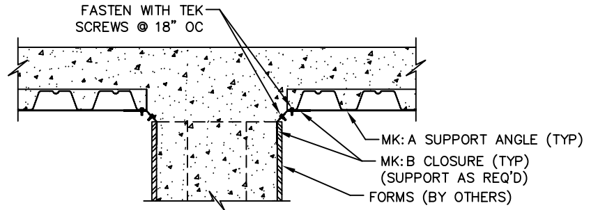
SECTION @ INT. DIAPHRAGM
