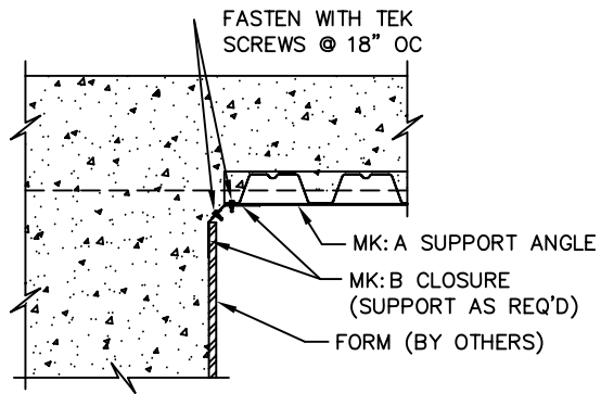
SECTION @ ABUTMENTS
